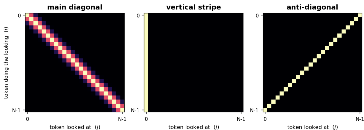
Figure 3: The three shapes, drawn by hand rather than taken from a model. A trained head may show one of them, a mixture, or nothing recognisable at all.
